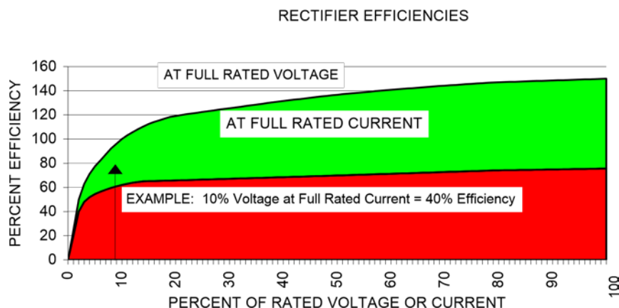
Figure 12. Rectifier Efficiency
