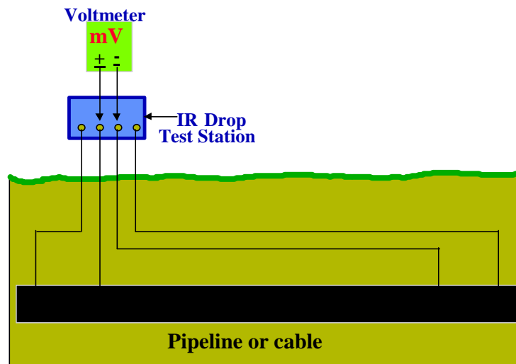
Figure 33 Typical IR Drop Test Span Installation
