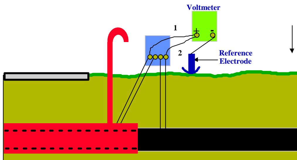
Figure 18 Testing for a Shorted Casing
